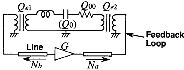
Fig. 1. Equivalent circuit of the AFR.
