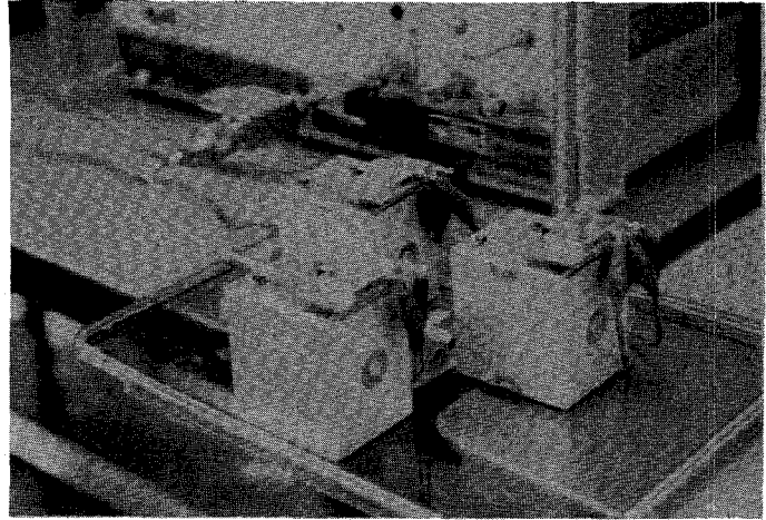
Fig. 13. NF measuring system for three-pole AFR BEF.
