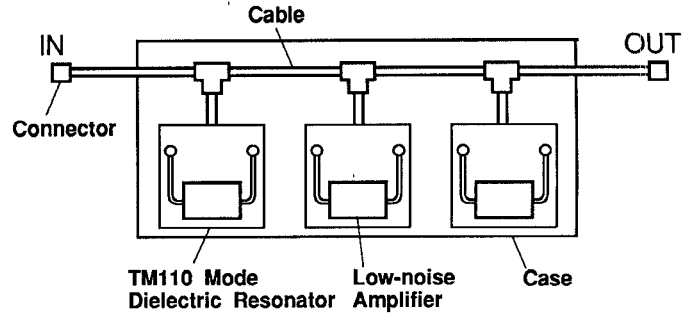
Fig. 5. Construction of the three-pole AFR BEF.
