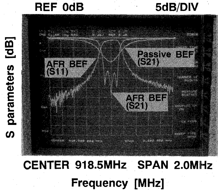
Fig. 14. S parameters of the three-pole AFR BEF.
