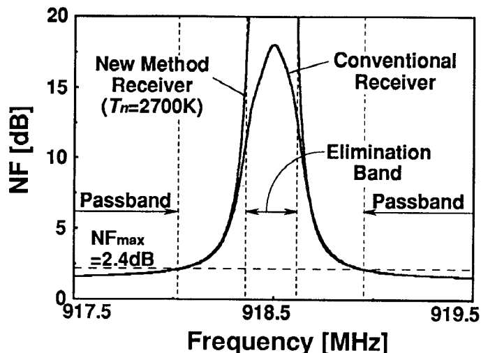
Fig. 11. Total NF of the receiver.
