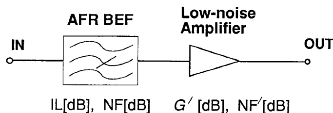
Fig. 10. Block diagram of receiver.
