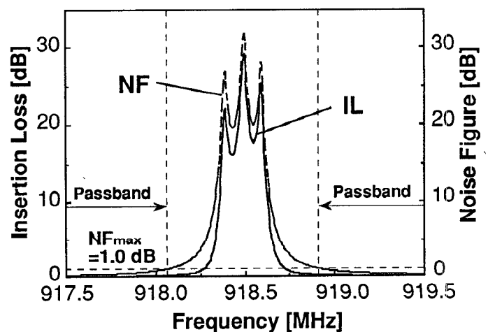
Fig. 7. NF estimation of the three-pole AFR BEF.
