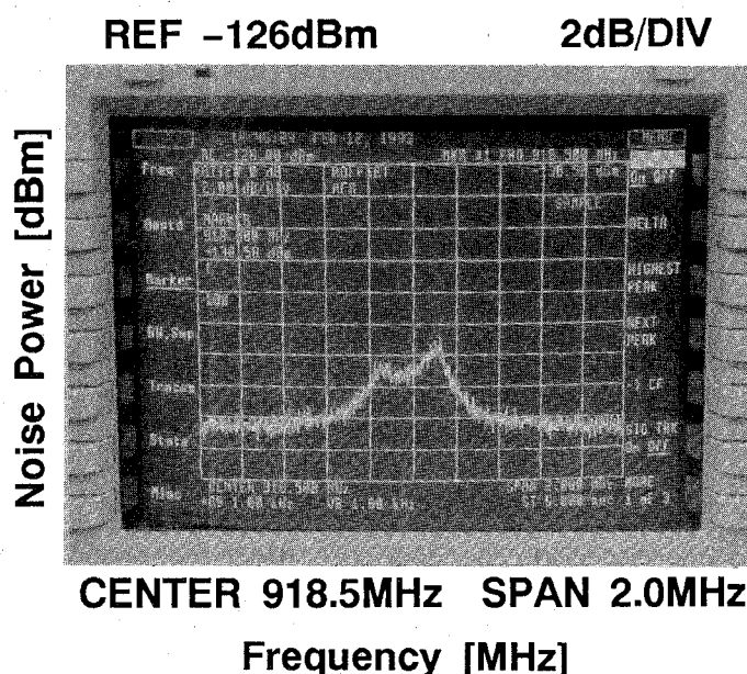
Fig. 15. Noise output of the three-pole AFR BEF.
