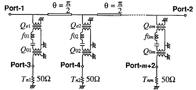
Fig. 4. Equivalent conversion of BEF circuit.
