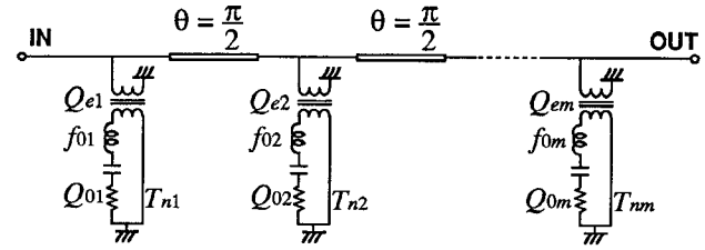
Fig. 3. Equivalent circuit of AFR BEF.
